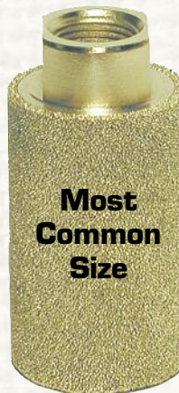
Part # CRY-ACC38PS 3/8" FNPT x 1 3/8" OD x 2 3/4" L
